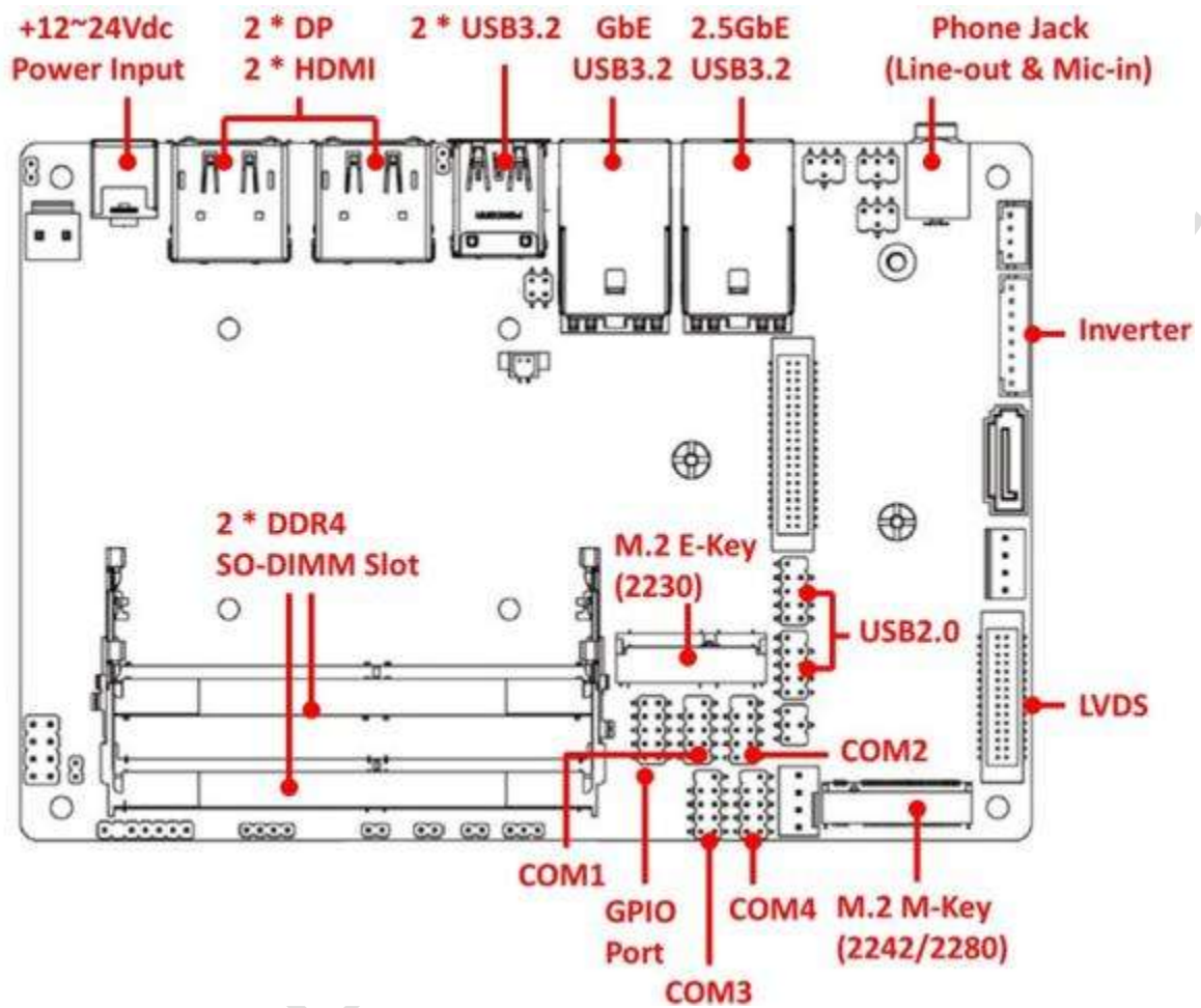
PPC TGL CPU Board
